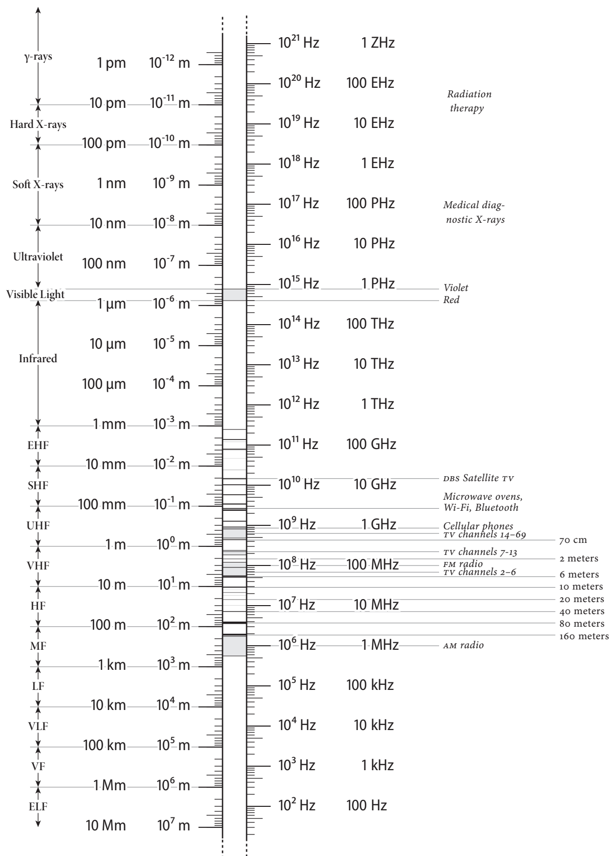
The Electromagnetic Spectrum
